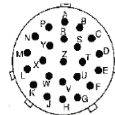
Shell Size 18 23
