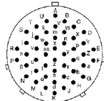
Shell Size 24 48
